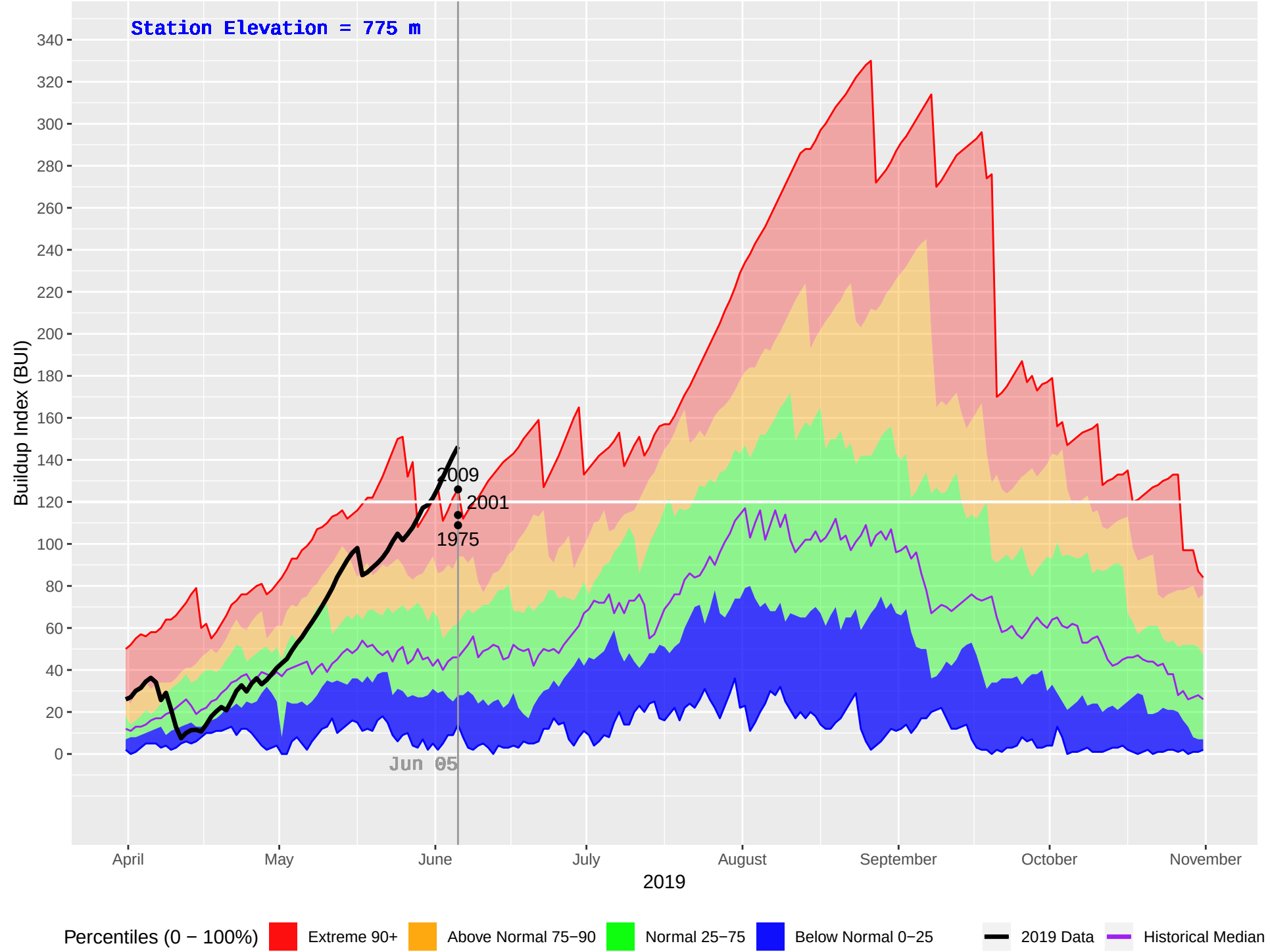
ELKO (412) : Historical (1970–2018), Current (2019) Daily Buildup Index (BUI)
