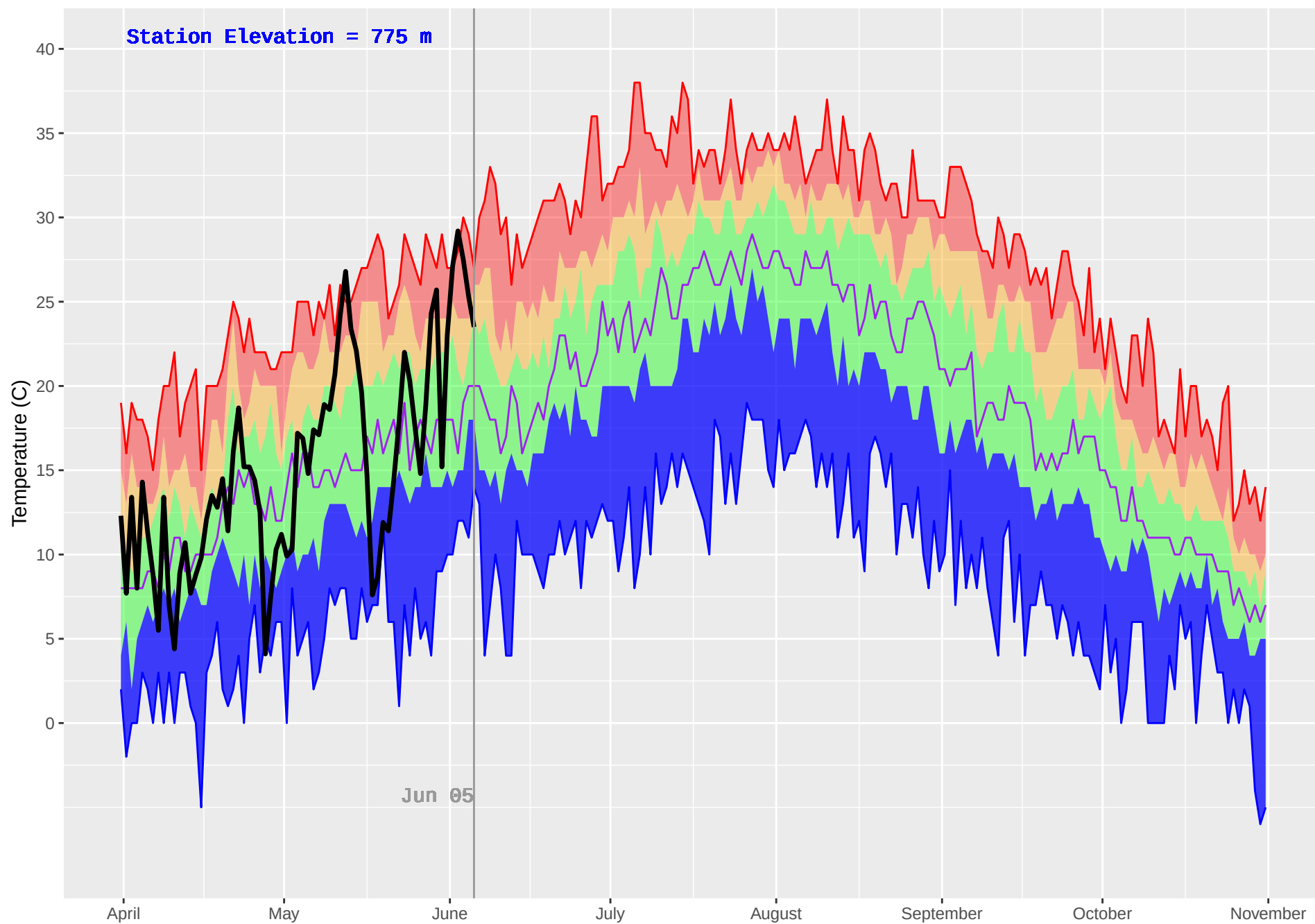
ELKO (412) : Historical (1970–2018) and Current (2019) Daily Temperature
