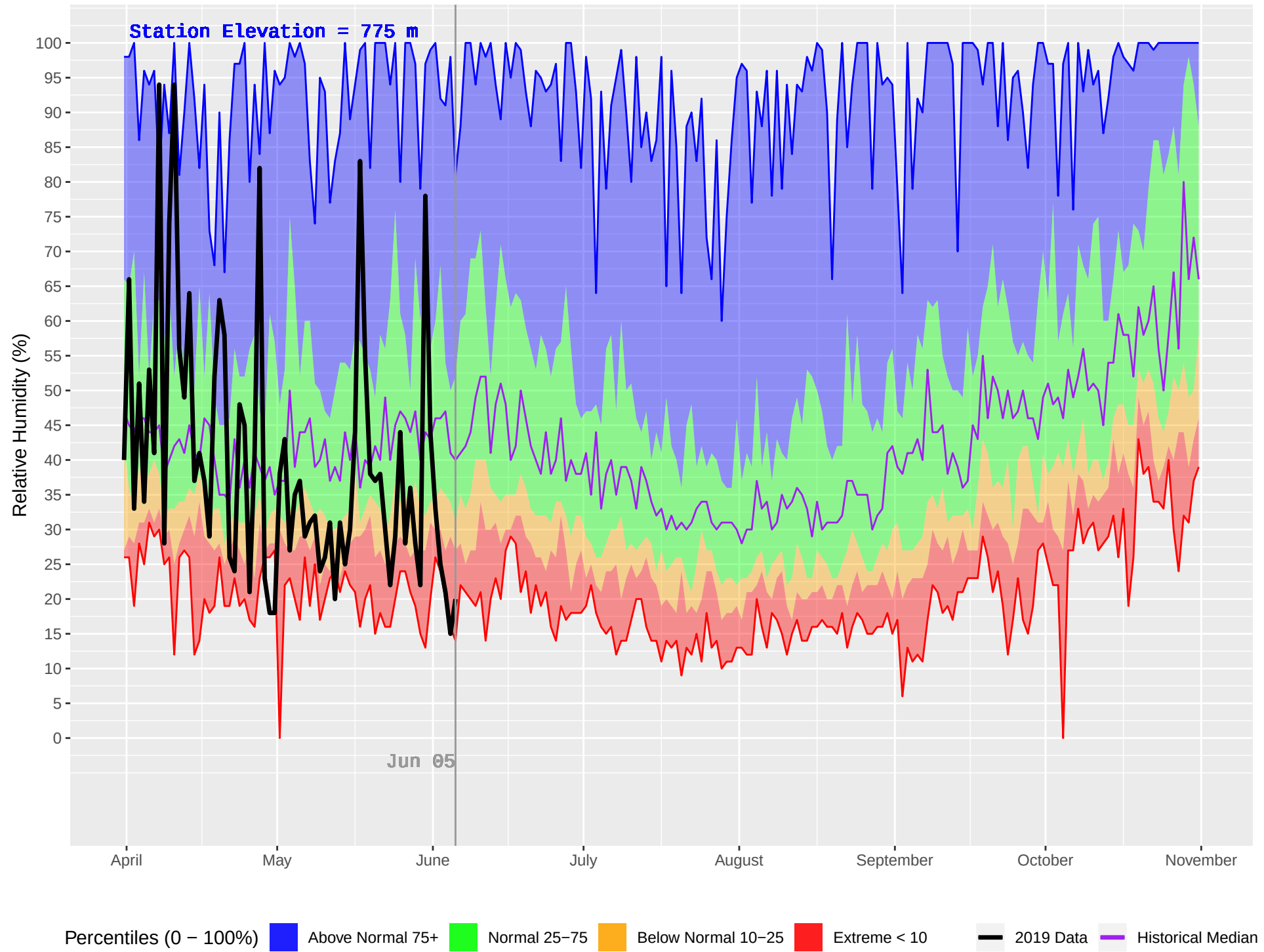
ELKO (412) : Historical (1970–2018) and Current (2019) Daily Relative Humidity
