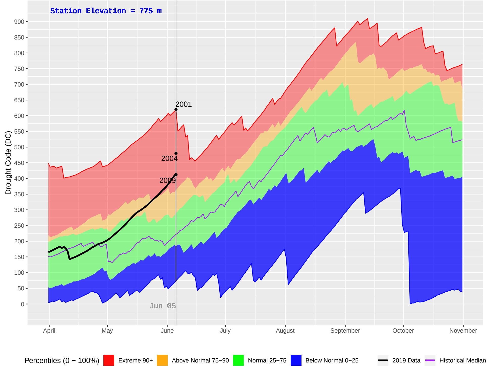
ELKO (412) : Historical (1970–2018) and Current (2019) Daily Drought Code (DC)
