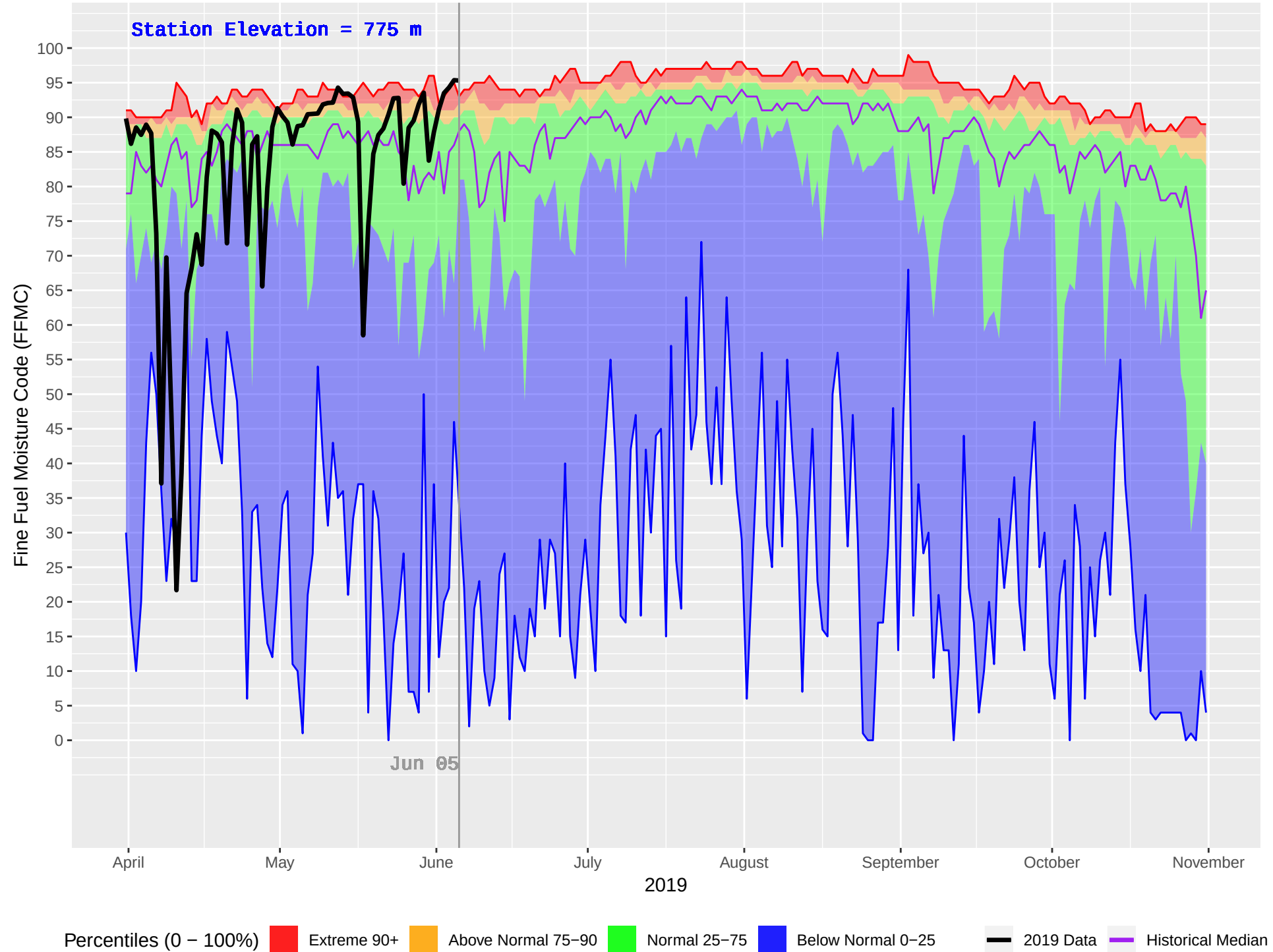
ELKO (412) : Historical (1970–2018) and Current (2019) Daily Fine Fuel Moisture Code (FFMC)
