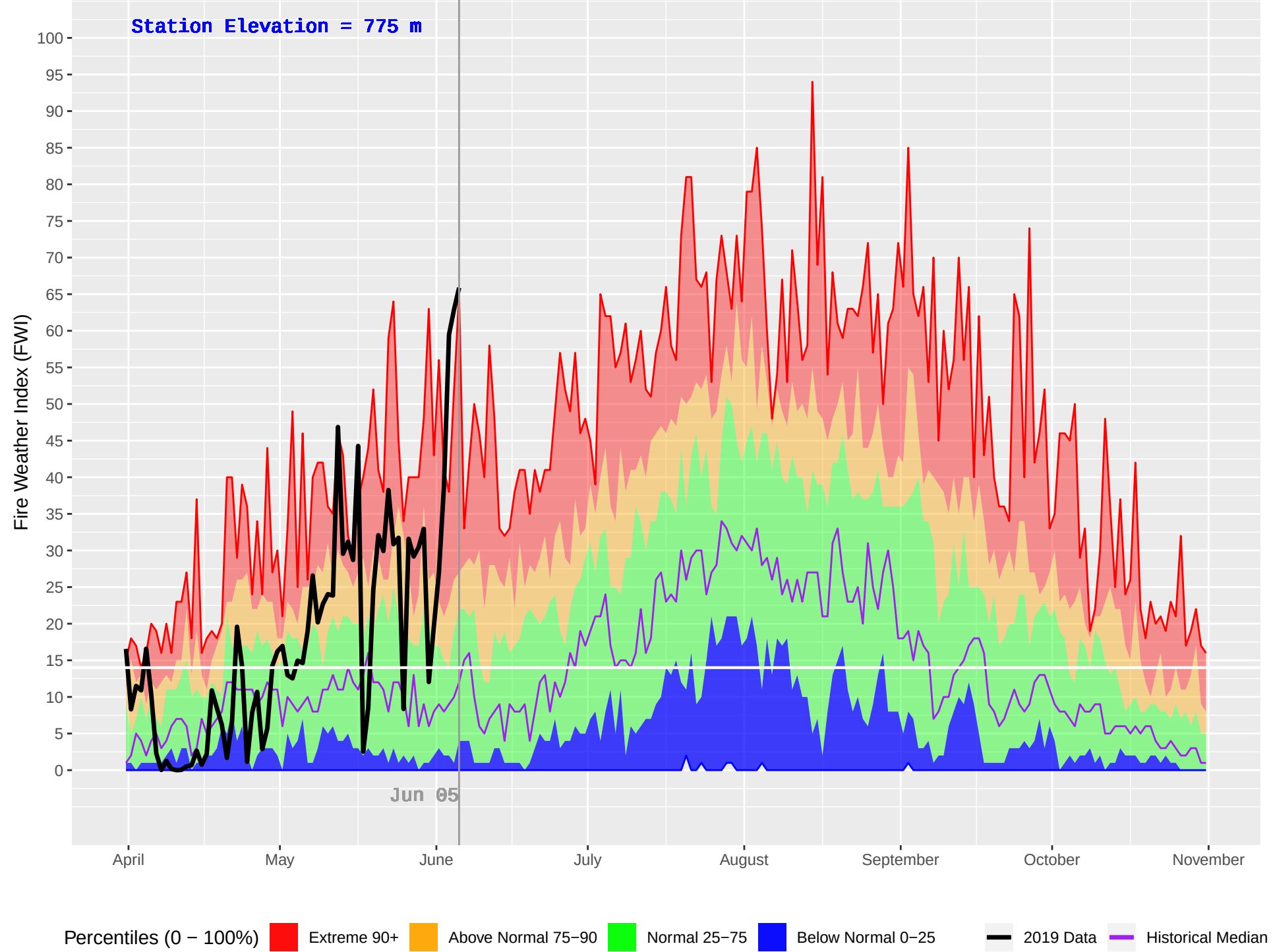
ELKO (412) : Historical (1970–2018) and Current (2019) Daily Fire Weather Index (FWI)
