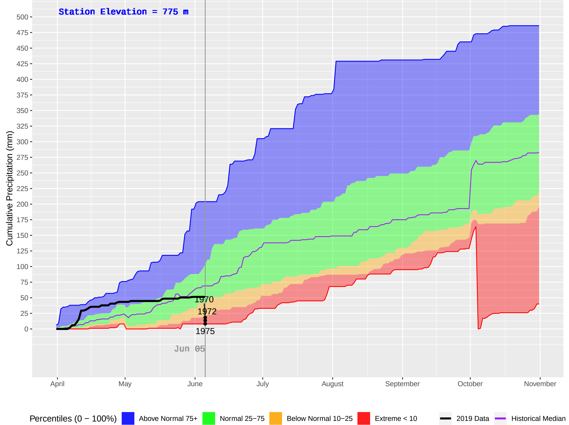
ELKO (412) : Historical (1970–2018), Current (2019) Daily Cumulative Precipitation
