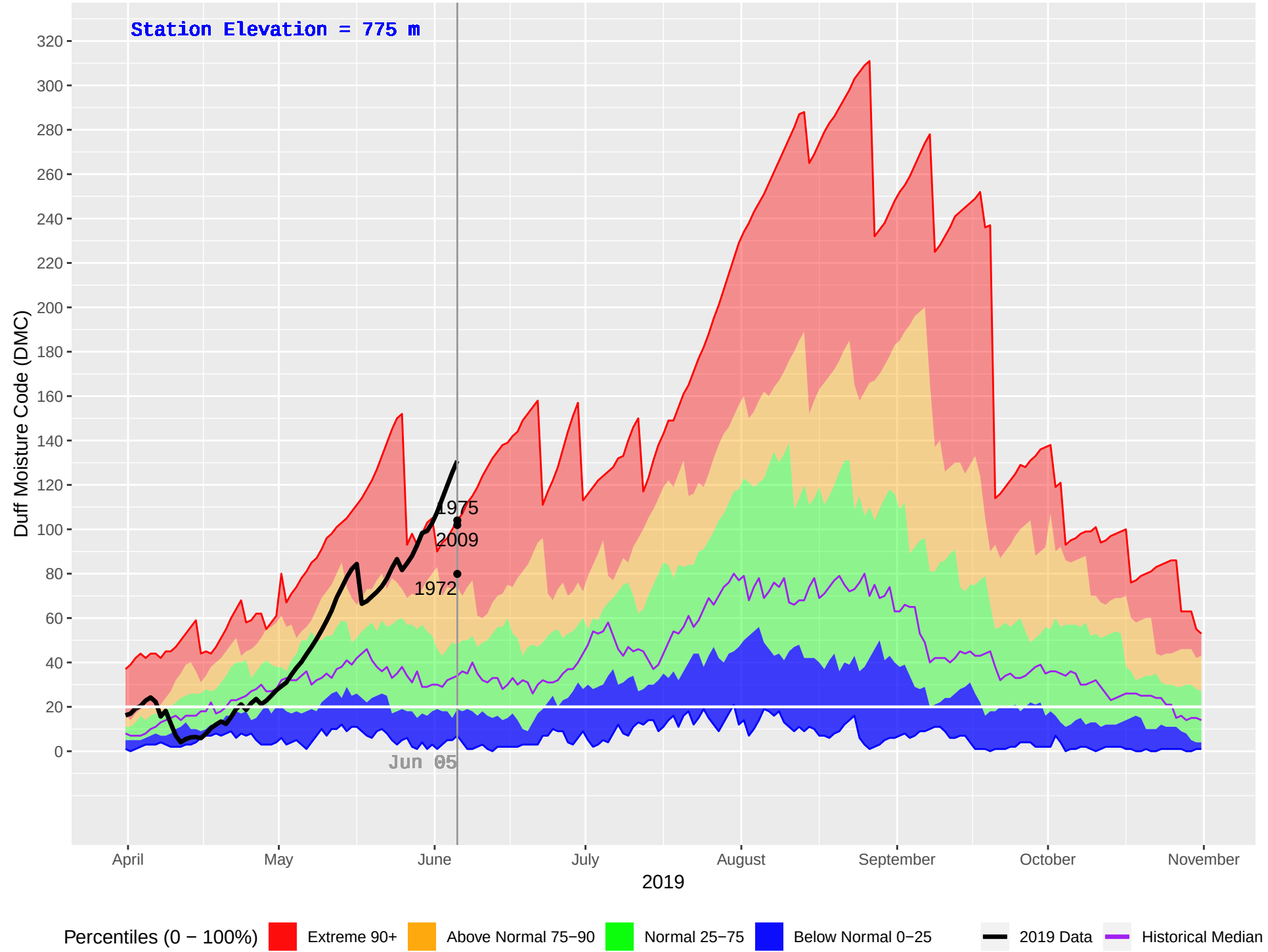
ELKO (412) : Historical (1970–2018), Current (2019) Daily Duff Moisture Code (DMC)
